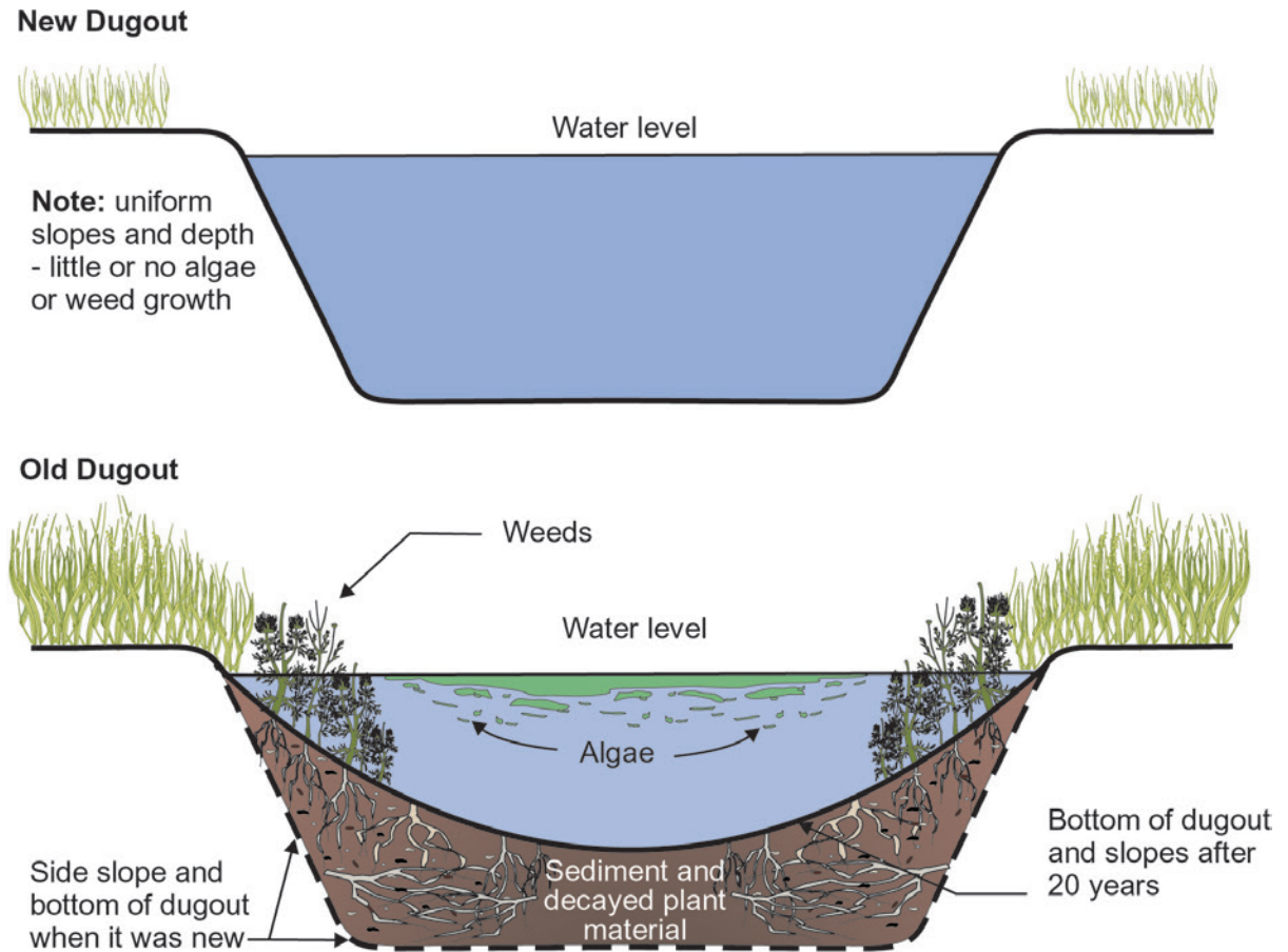
Figure 2-8 New vs. Old Dugout Cross-sections
