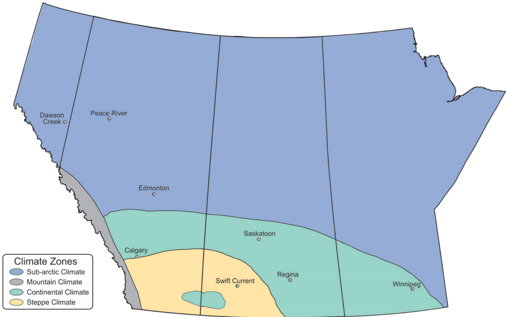
Figure 2-1 Climate Zones
