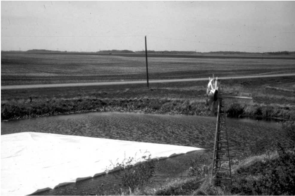
Figure 8-5 Dugout Cover
