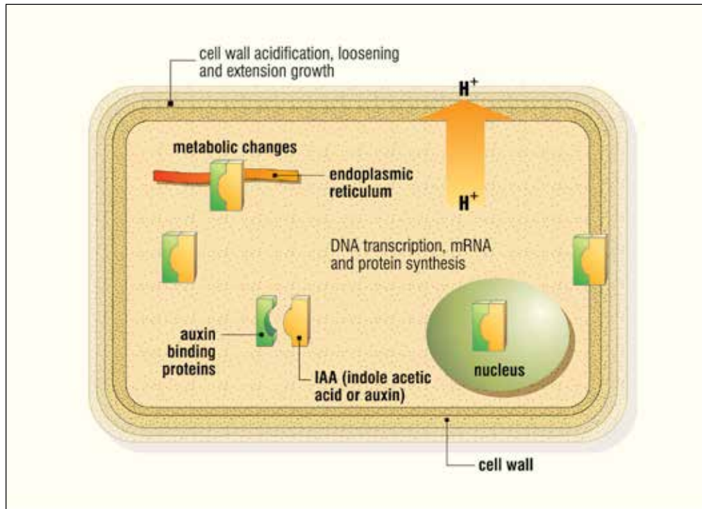
Figure 36. Auxin binding proteins have been identified in several locations: on the plasma membrane, dissolved in the cytoplasm and in the nucleus and endoplasmic reticulum (ER). Auxin binding causes a rapid efflux of protons, followed by cell wall loosening. Loosening of the bonds between the cell wall fibers allows the cell to increase in size. This action is called the 'acid growth phase'. Slower responses include enzyme induction, nuclear transcription, mRNA and protein and polysaccharide synthesis.
