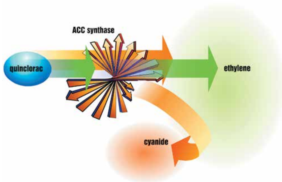
Figure 38. A secondary effect of quinclorac has recently been identified in grass weeds. In the presence of quinclorac, the enzyme ACC synthase increases activity, producing a large increase in ethylene, up to 60 times the normal amount. A by-product of ethylene biosynthesis is cyanide, a metabolic inhibitor.
