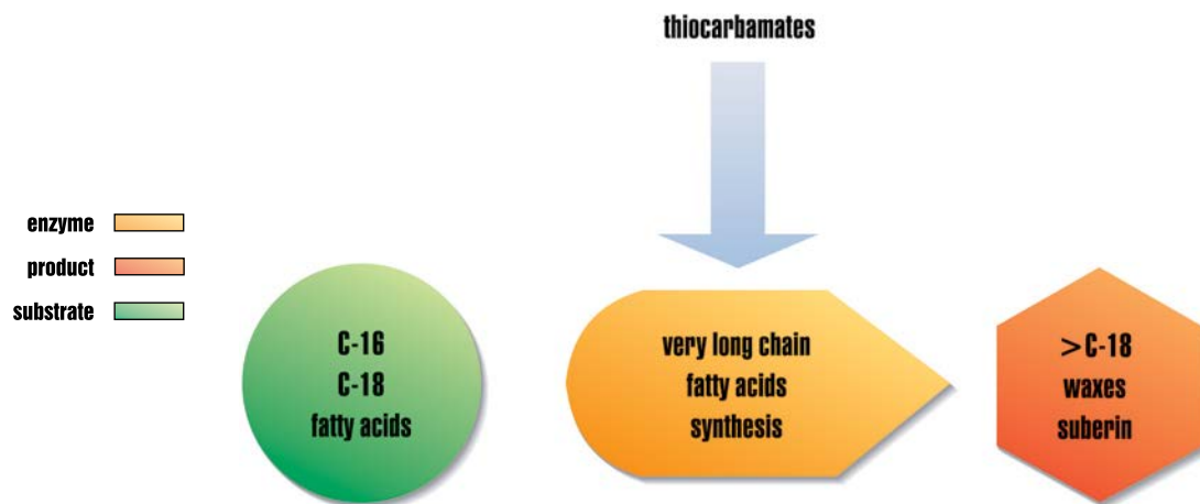
Figure 17. The thiocarbamates inhibit the synthesis of very long chain fatty acids (carbon chain length greater than 18) and block production of waxes and suberin.
