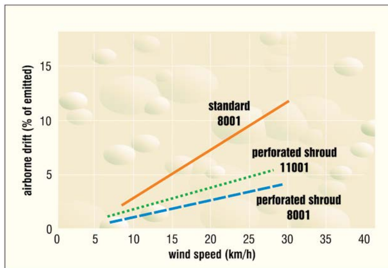
Figure 80. Reduction of drift with shrouds. Application volume was 50 L/ha.
