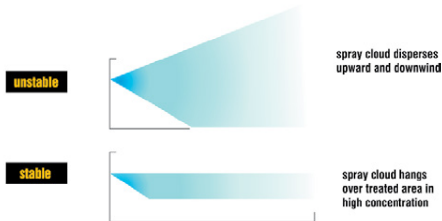
Figure 73. Fate of a spray cloud under unstable and stable (inversion) conditions. Source 8
