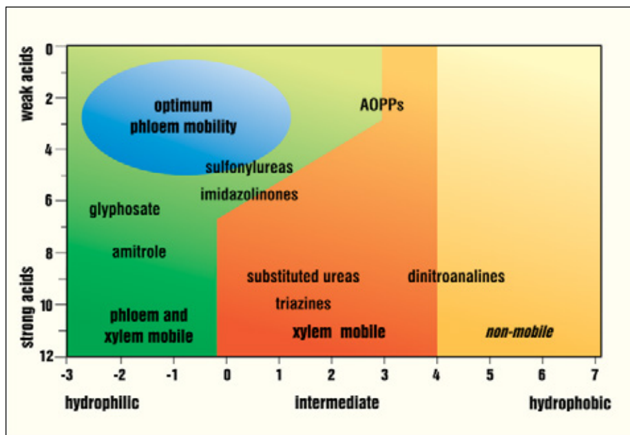
Figure 5. The influence of solubility and acid nature of common herbicides on translocation in both phloem and xylem.
