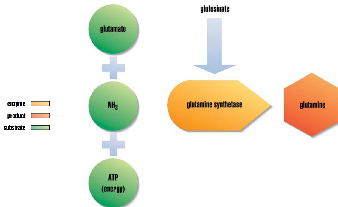
Figure 28. Glufosinate inhibits glutamine synthetase, an enzyme that combines inorganic \text{NH}_3 with glutamate to form glutamine.
