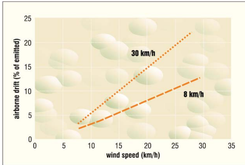
Figure 79. Effect of travel speed on spray drift: 30 km/h travel speed conducted using XR11002 tips applying 30 L/ha and 8 km/h travel speed done using XR8001 tips applying 50 L/ha.
