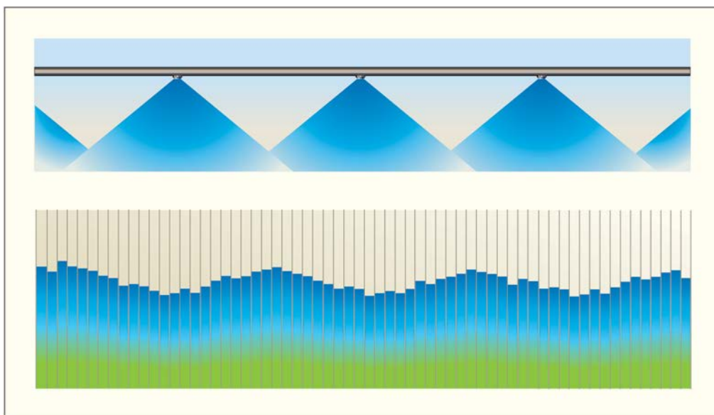
Figure 60. A typical static spray pattern.
