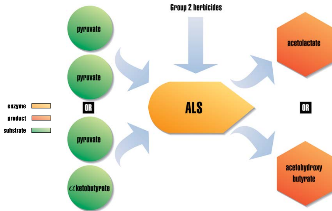
Figure 21. All Group 2 herbicides inhibit acetolactate synthase (ALS/AHAS). Enzyme inhibition leads to an accumulation of \alpha ketobutyrate, a reduction in protein synthesis and eventually to plant death.
