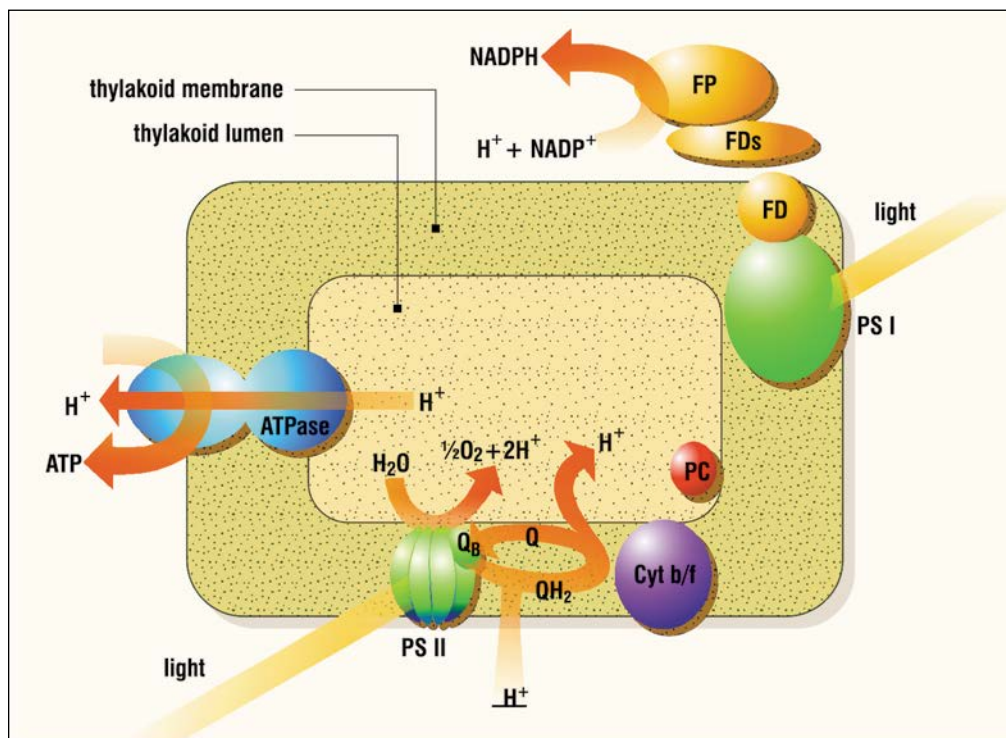
Figure 42. The light reactions of photosynthesis require movement of electrons from PS II, through QB, to Cytochrome b/f, to a plastiquinone (PC) then finally through PS I and several iron containing carriers, FD, FDs and FP. Electron movement transports protons, leading to ATP production, synthesizes NADPH and creates oxygen as a by-product.
