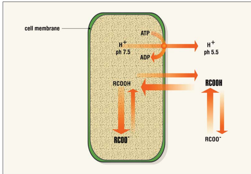
Figure 3. Acid trapping of weak acid herbicides.
