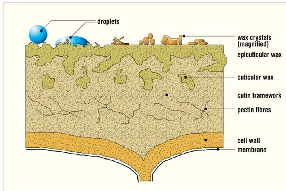
Figure 72. Cross-section of a leaf cuticle showing epicuticular and cuticular waxes and cutin, which represent a barrier to herbicide entry into plant cells.
