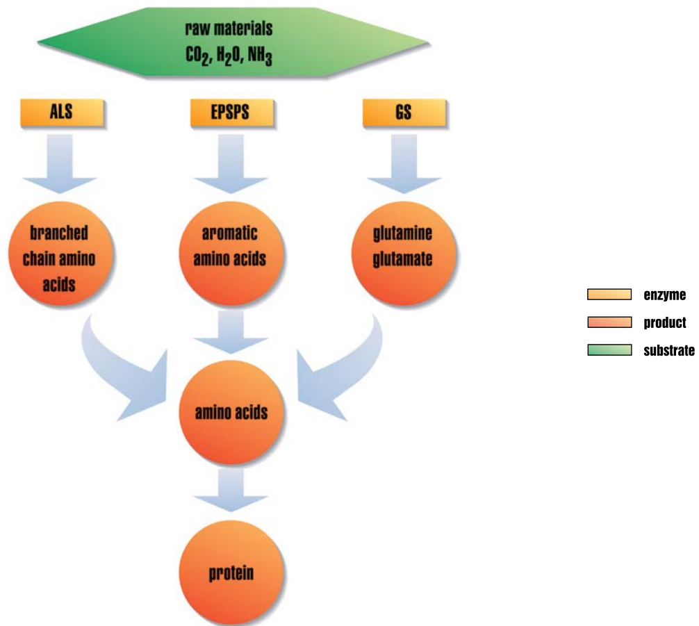
Figure 19. Three different groups of herbicides inhibit amino acid biosynthesis.
