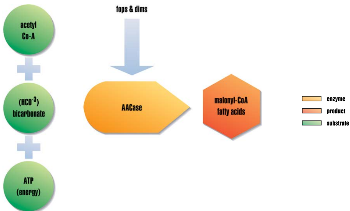
Figure 31. Group 1 herbicides inhibit the enzyme ACCase, critical to the formation of fatty acids.
