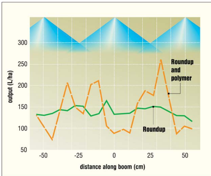
Figure 78. Effect of a drift-reducing adjuvant on the spray pattern of Roundup. Nozzle was an XR8003 at 40 psi pressure, traveling at 8 km/h. Source 10
