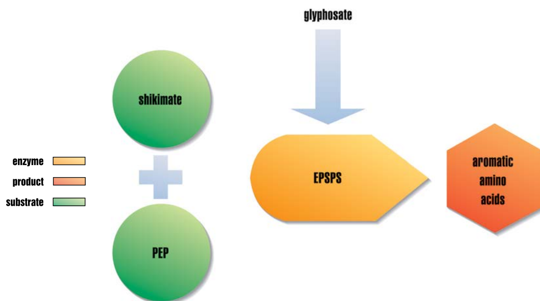
Figure 25. Glyphosate inhibits a key enzyme in aromatic amino acid biosynthesis.
