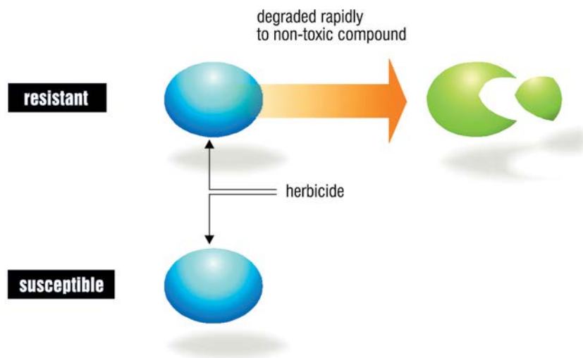
Figure 52. Some resistant weeds can rapidly degrade the herbicide to a non-toxic compound while the susceptible weeds cannot. In susceptible weeds, the herbicide remains in the toxic form.
