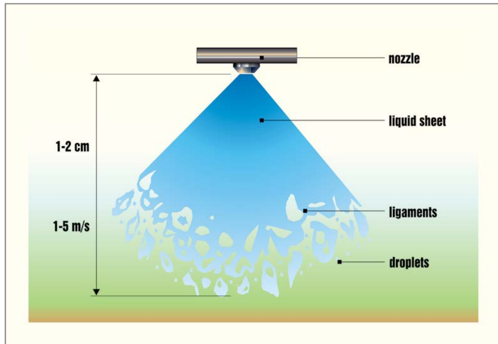
Figure 55. Sheet breakup in a flat fan nozzle – from a solid liquid sheet – becoming unstable, forming ligaments and finally breaking into droplets.
